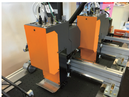
Print Head Modules Mounted on Supports
